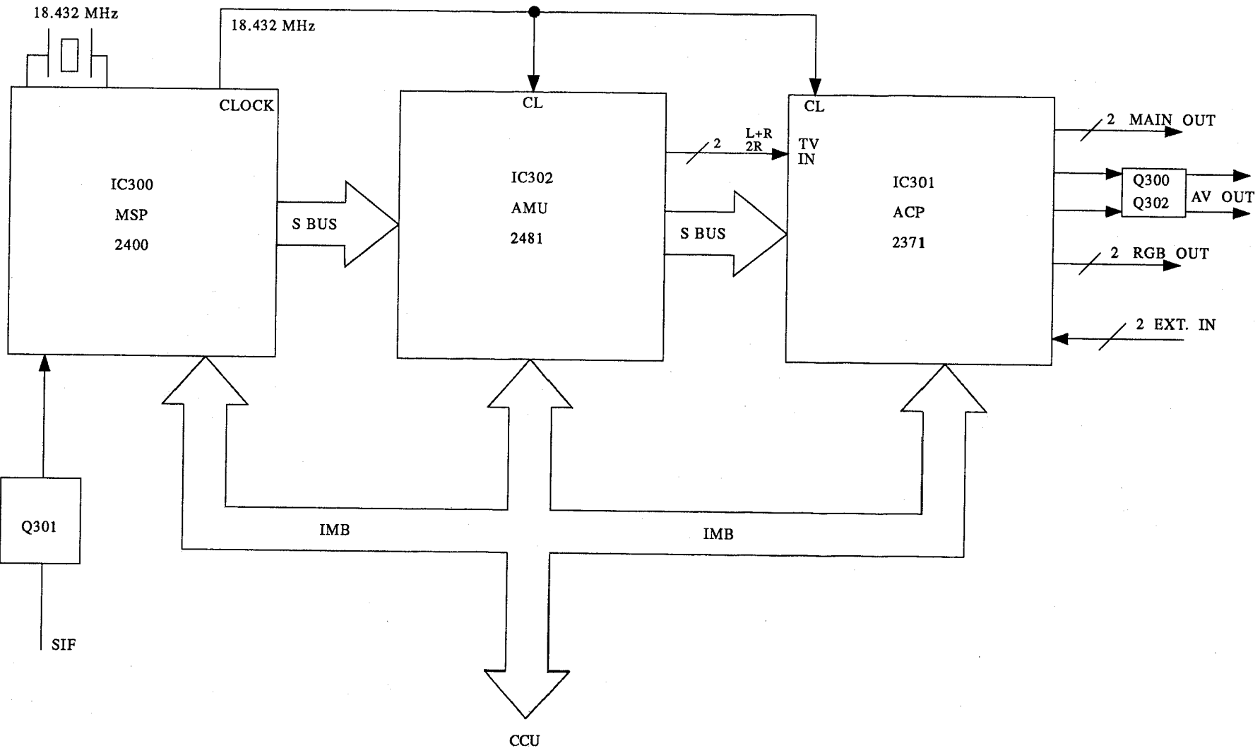
BLOCK DIAGRAM NICAM UNIT
